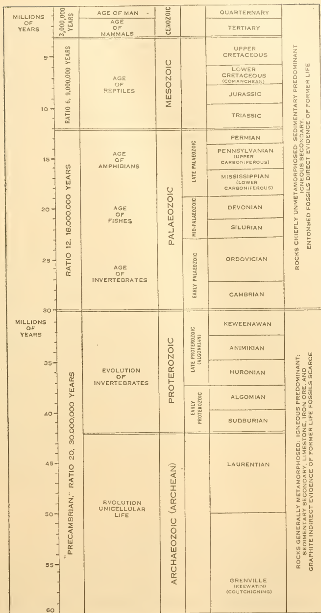
Fig. 30.—Total geologic time scale, estimated at sixty million years. (From Newman, after Osborn.)
