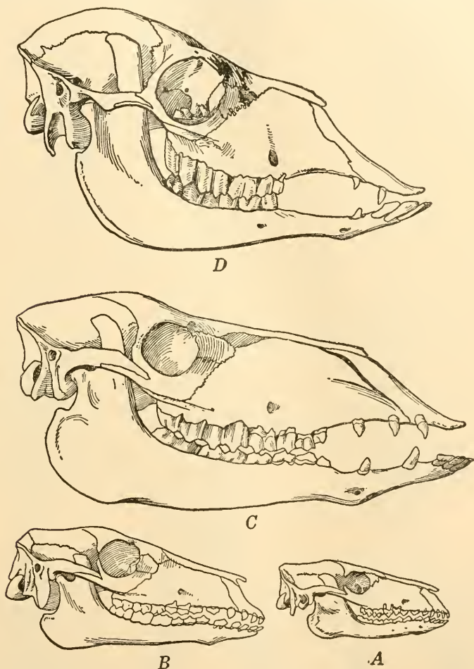
FIG. 32.—Four stages in the evolution of the cameline skull. A , Protilyopus , Upper Eocene; B , Poebrotherium , Lower Oligocene; C , Procamelus , Upper Miocene; D , guanaco , Recent. (From Scott.)
