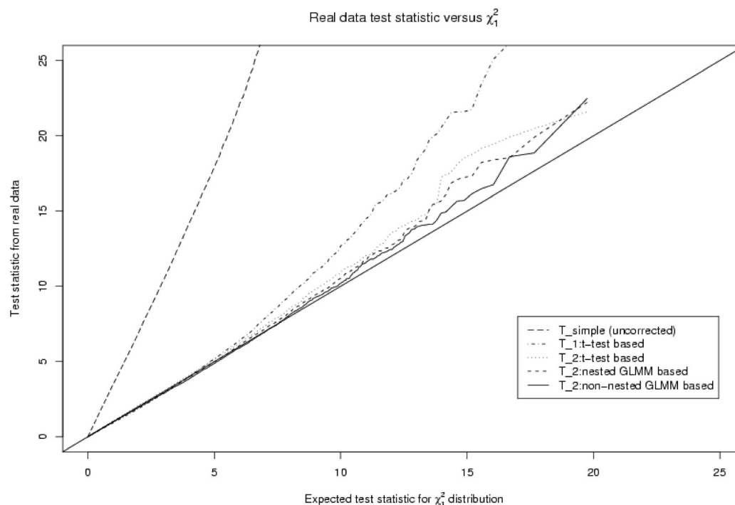
Figure 1. Comparison of test statistic performance. Results for 56 494 SNPs. Each statistic is plotted against the expected distribution under the hypothesis that there are no (or very few) true positives. A test statistic with distribution exactly equal to the expected asymptotic distribution will lie along the plotted y = x line. The plotted lines exhibit considerable stochastic variation at high values ( >18 ) because there are few data points in this range.
