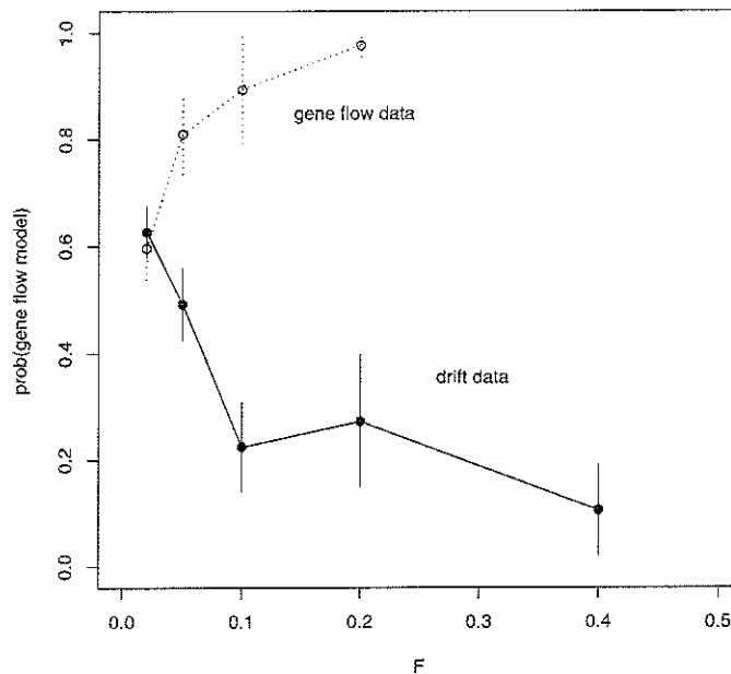
Fig. 2. p(I|D) plotted against F : the points are means based on five replicates and the vertical lines show estimates of the standard errors ( \circ , gene flow model; \bullet , transient model)
